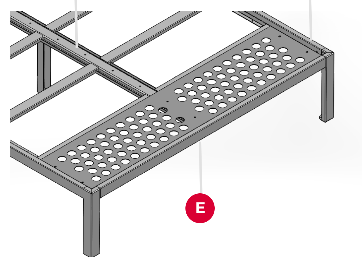
E to B Place Plate on Frame, line up holes in the plate with holes in the Side Bar and Middle Bar.
