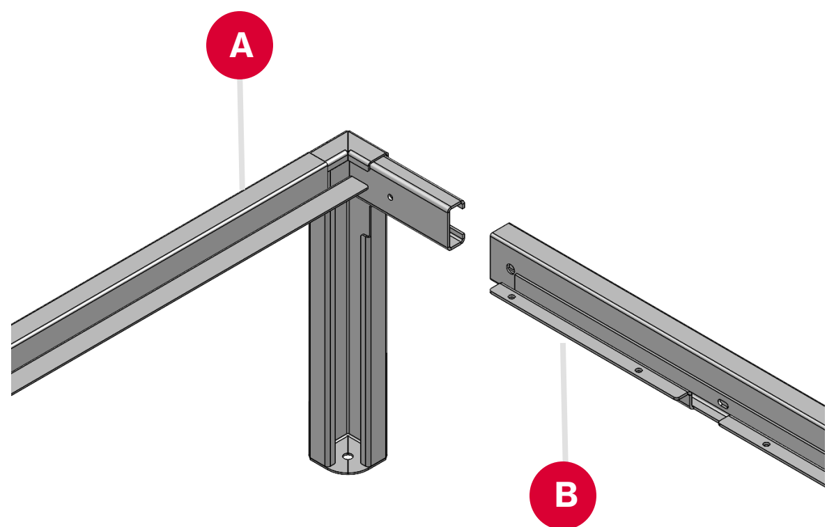
A to B Attach Side Bars to a Frame End
