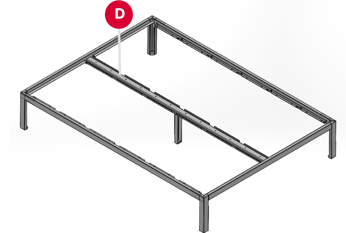
D to A Insert Middle Bar
