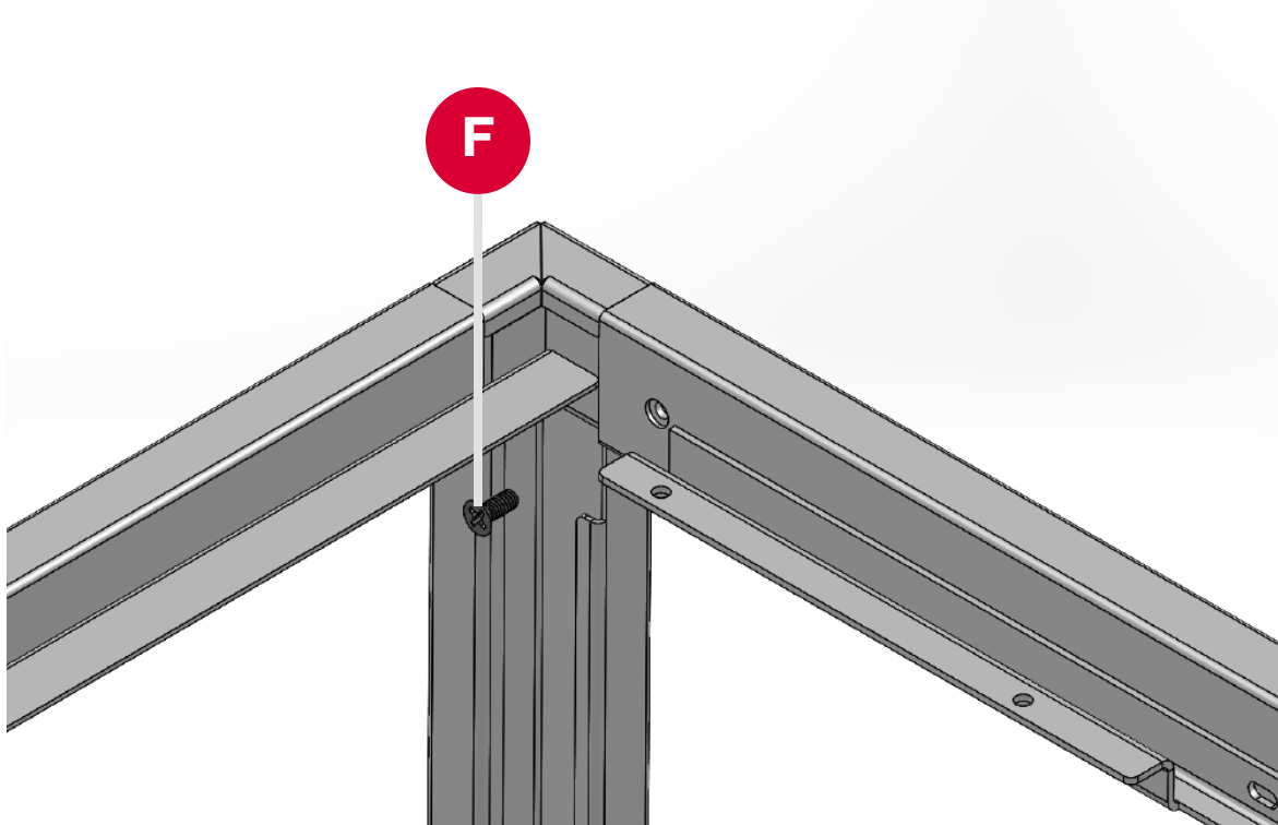
F to B Insert screw into corner hole and screw in with Phillips screwdriver
